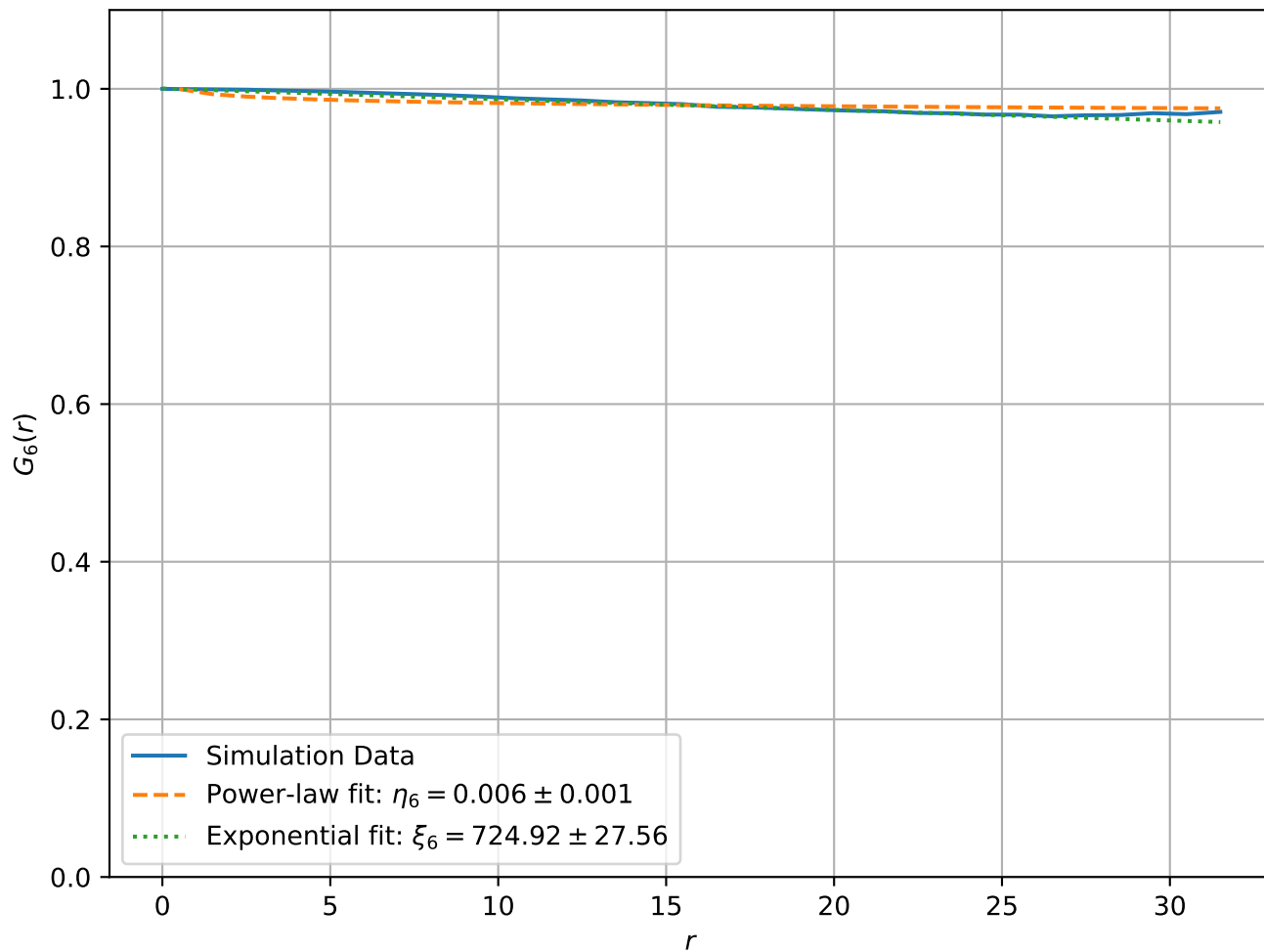
Correlation Function at T = 1.00\text{e} - 02 , L = 64
