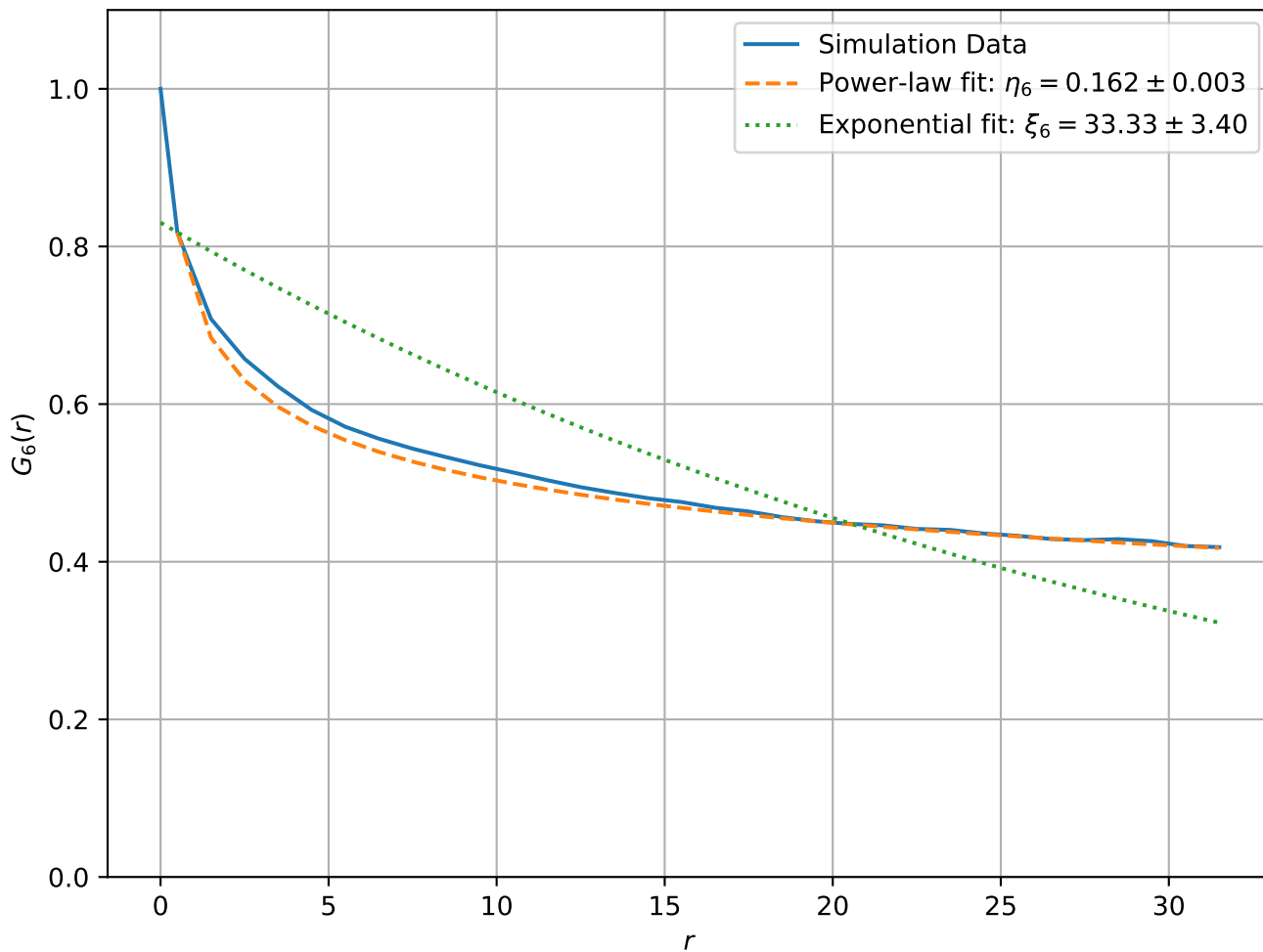
Correlation Function at T = 1.80e - 01 , L = 64
