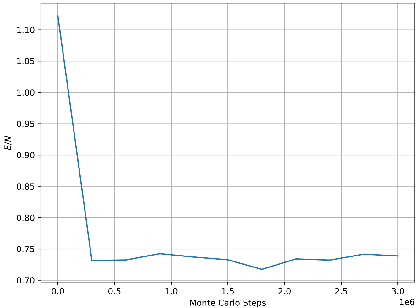
Energy per Spin at T = 2.10e - 01 , L = 64
