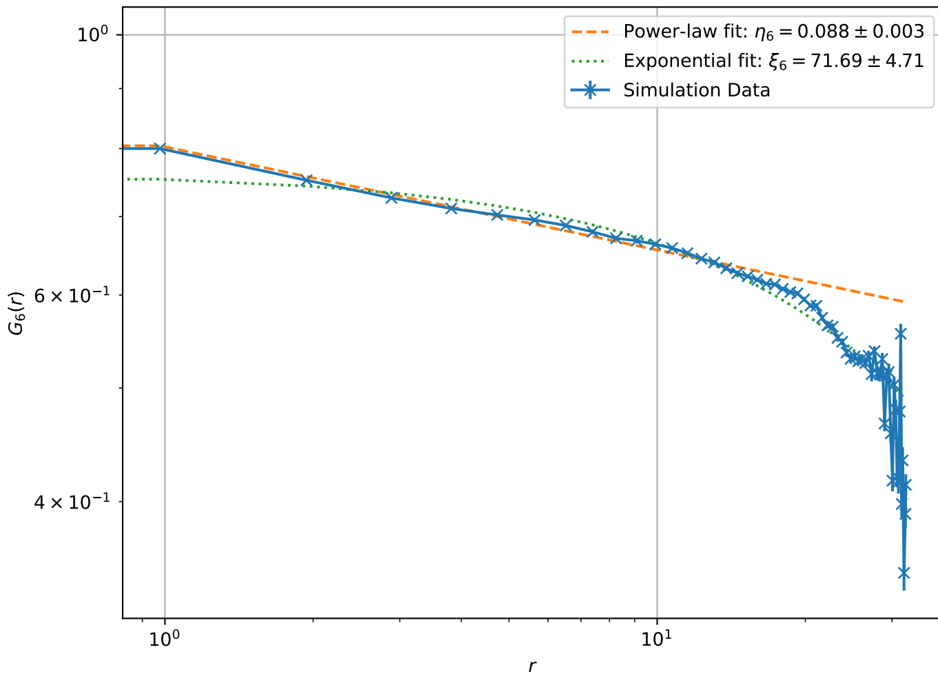
Correlation Function at T = 1.60e - 01 , L = 32 (Log-Log Scale)
