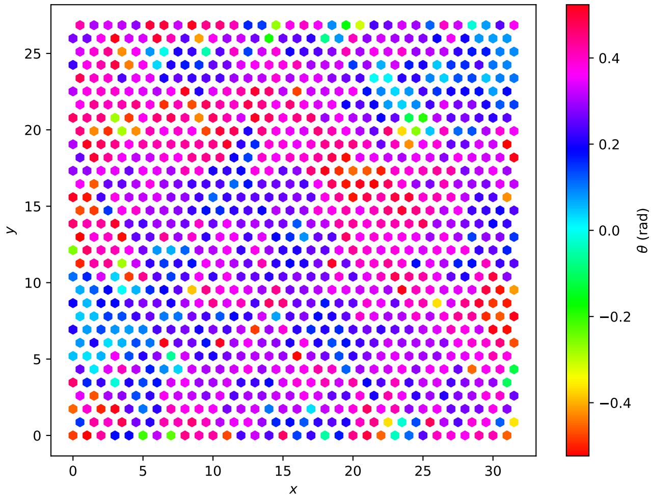
Hexagonal Lattice L=32 , T = 1.80e - 01
