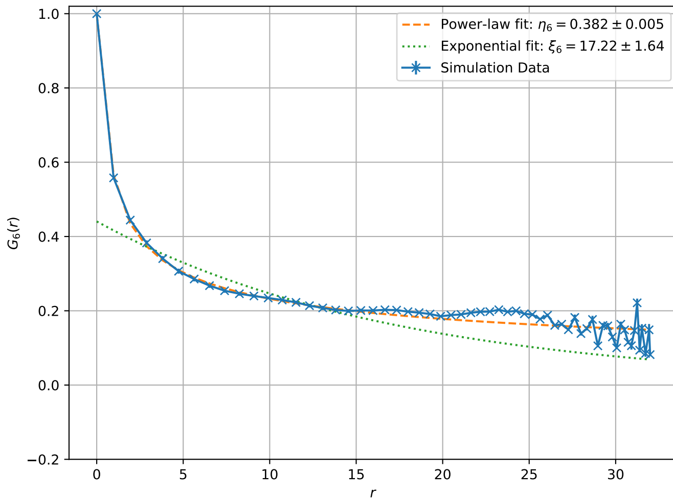
Correlation Function at T = 2.00e - 01 , L = 32
