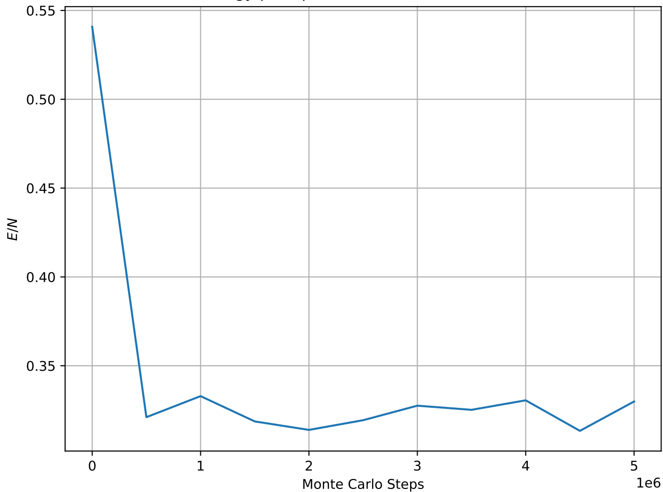
Energy per Spin at T = 2.00e - 01 , L = 32
