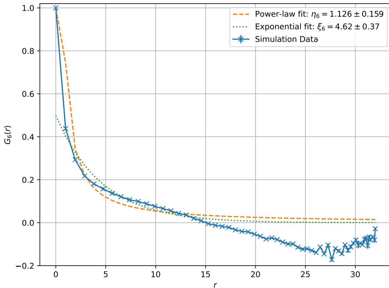
Correlation Function at T = 2.20e - 01 , L = 32
