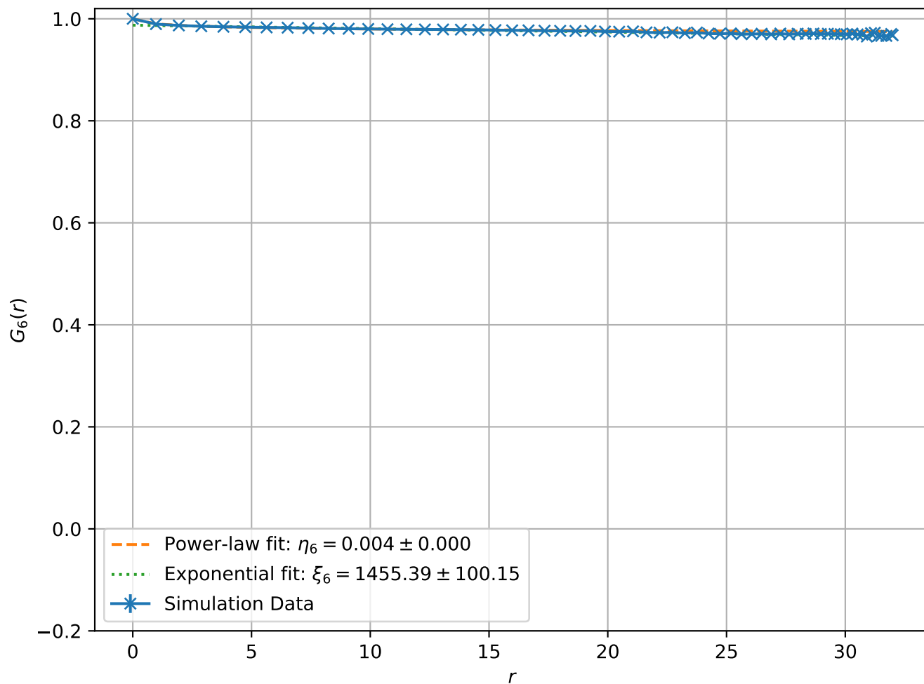
Correlation Function at T = 6.00e - 02 , L = 32
