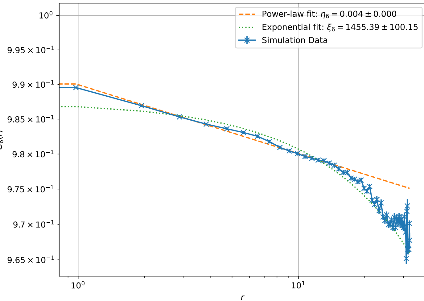
Correlation Function at T = 6.00e - 02 , L = 32 (Log-Log Scale)
