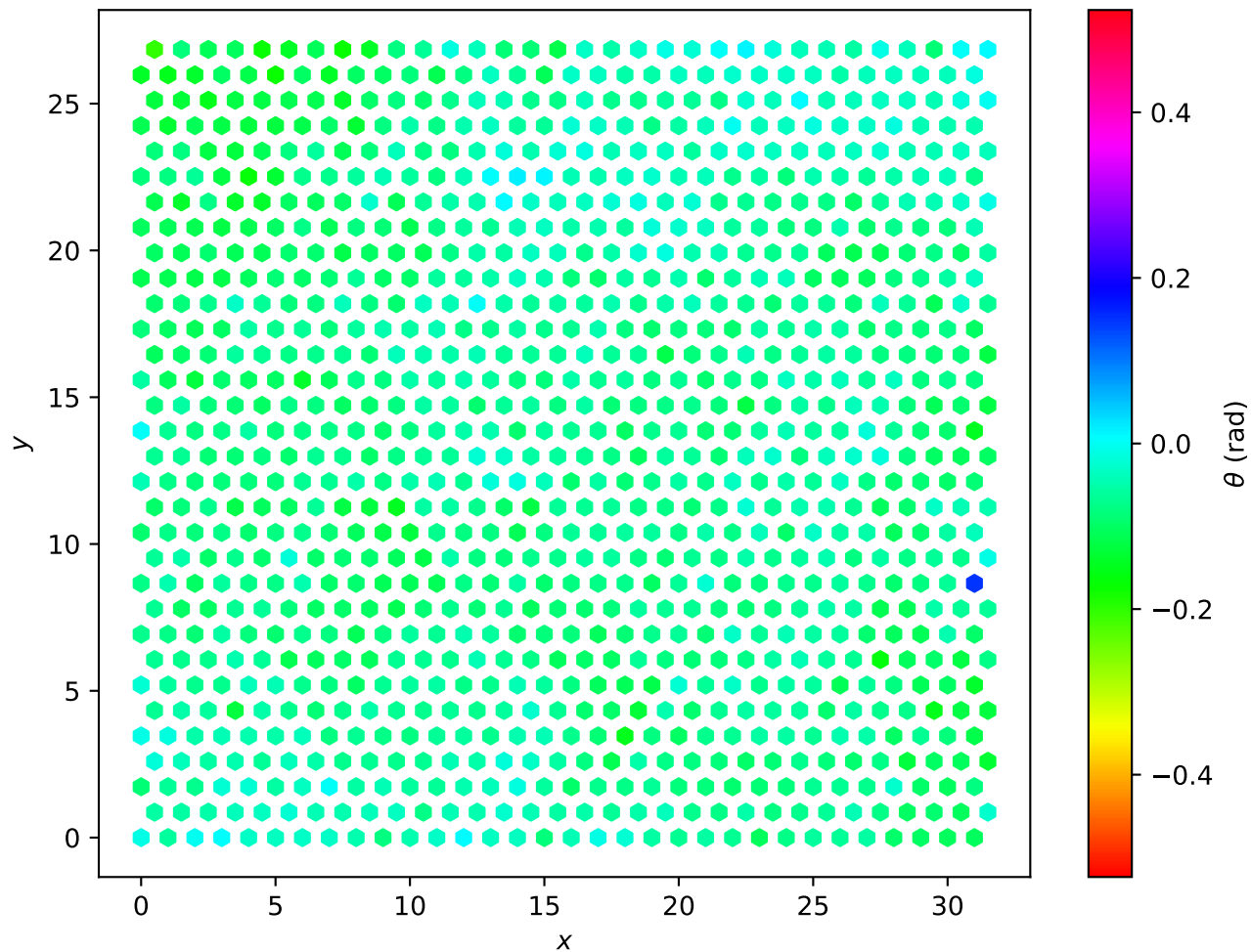
Hexagonal Lattice L=32 , T = 7.00e - 02
