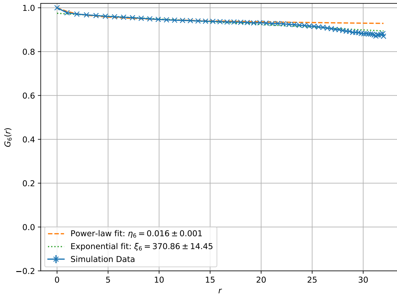
Correlation Function at T = 8.00e - 02 , L = 32
