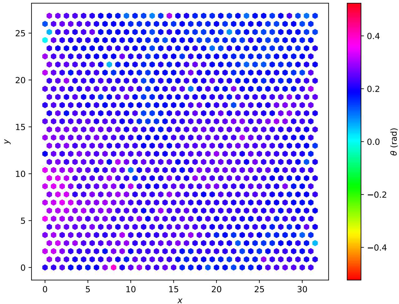
Hexagonal Lattice L=32 , T = 8.00e - 02
