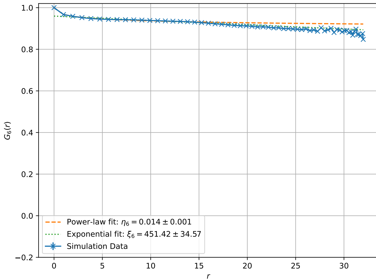
Correlation Function at T = 9.00e - 02 , L = 32
