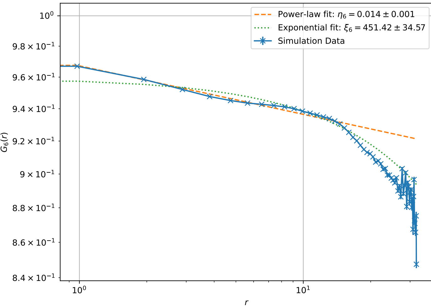
Correlation Function at T = 9.00e - 02 , L = 32 (Log-Log Scale)
