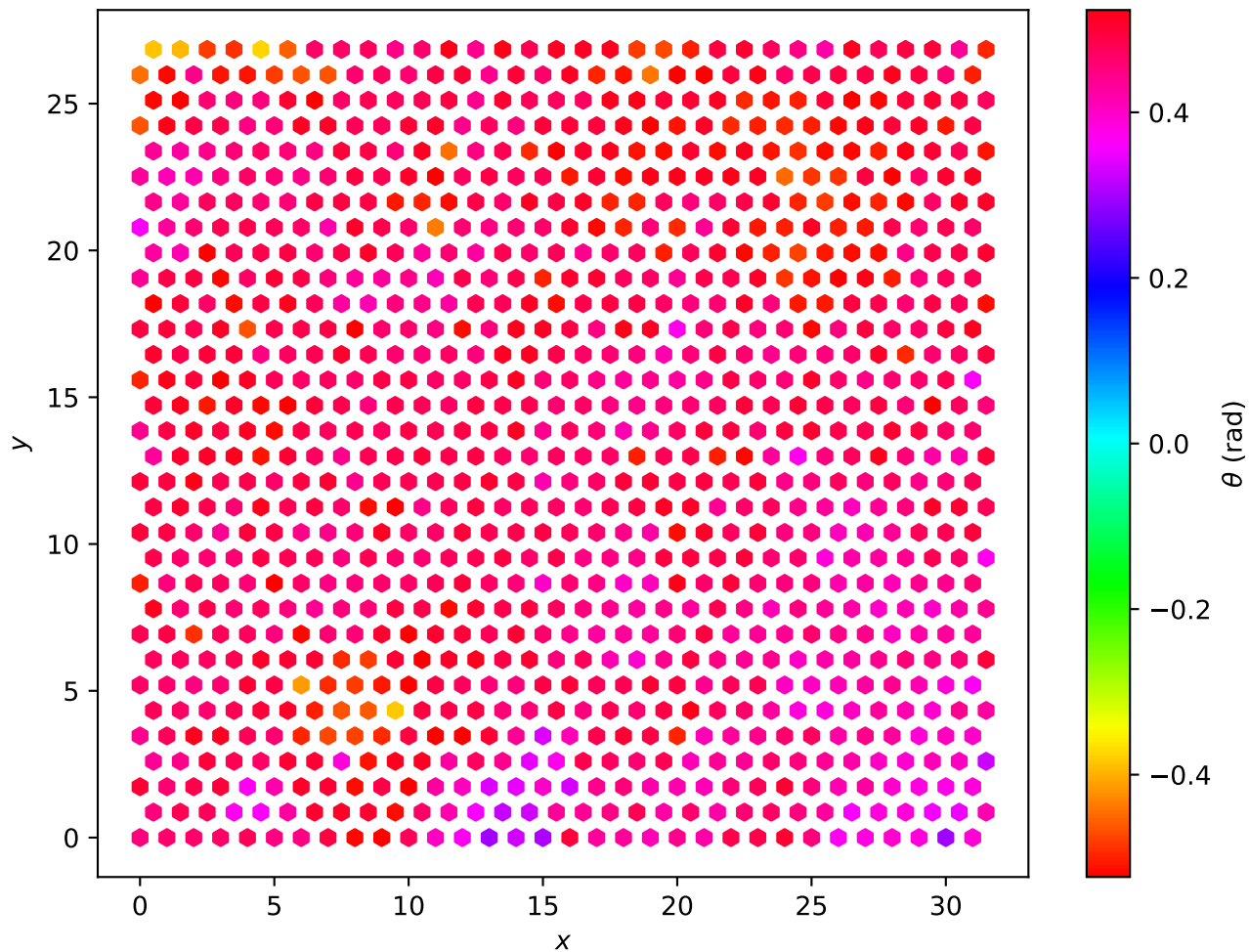
Hexagonal Lattice L=32 , T = 9.00e - 02
