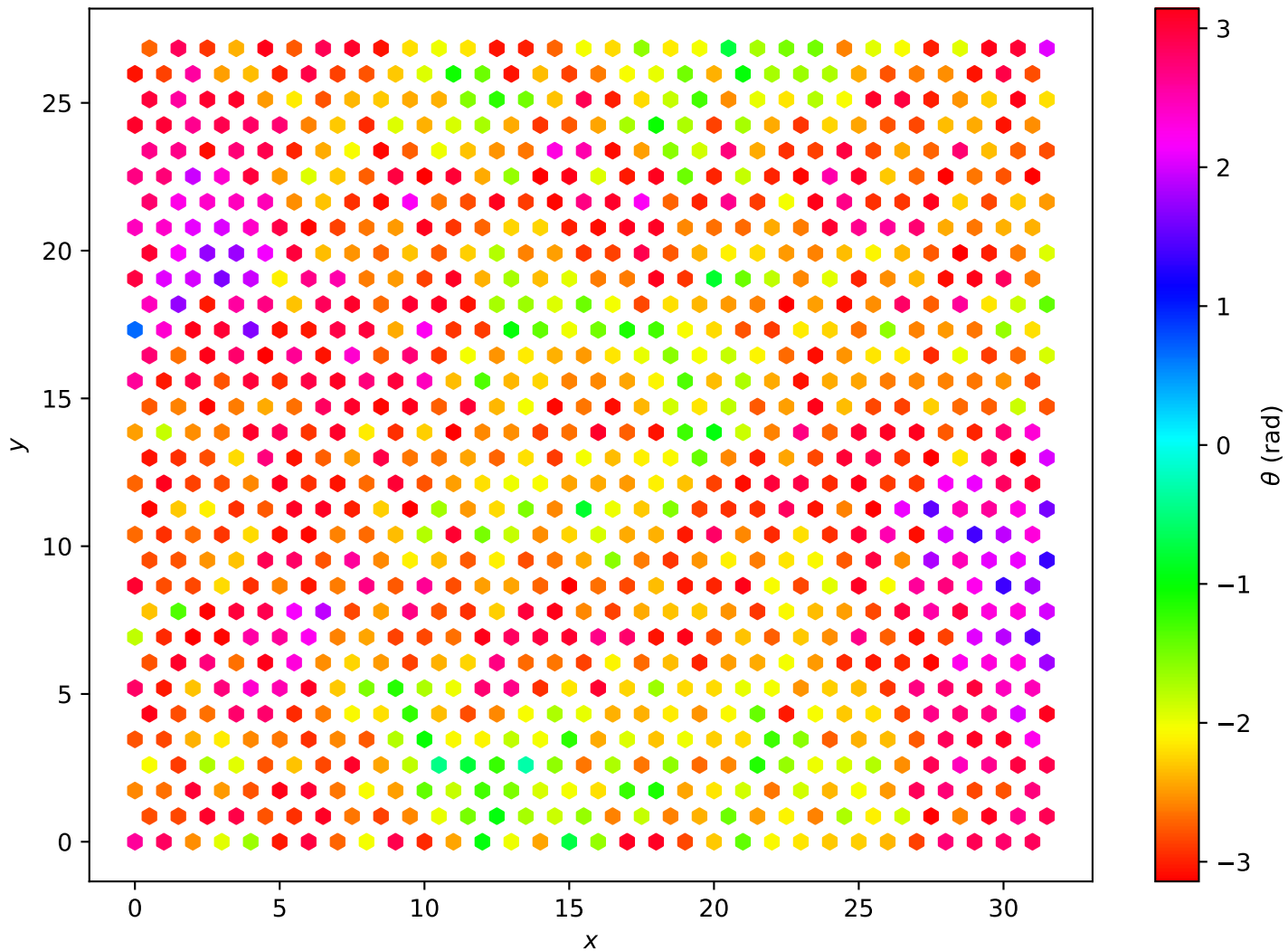
Hexagonal Lattice L=32 , T = 1.00e + 00
