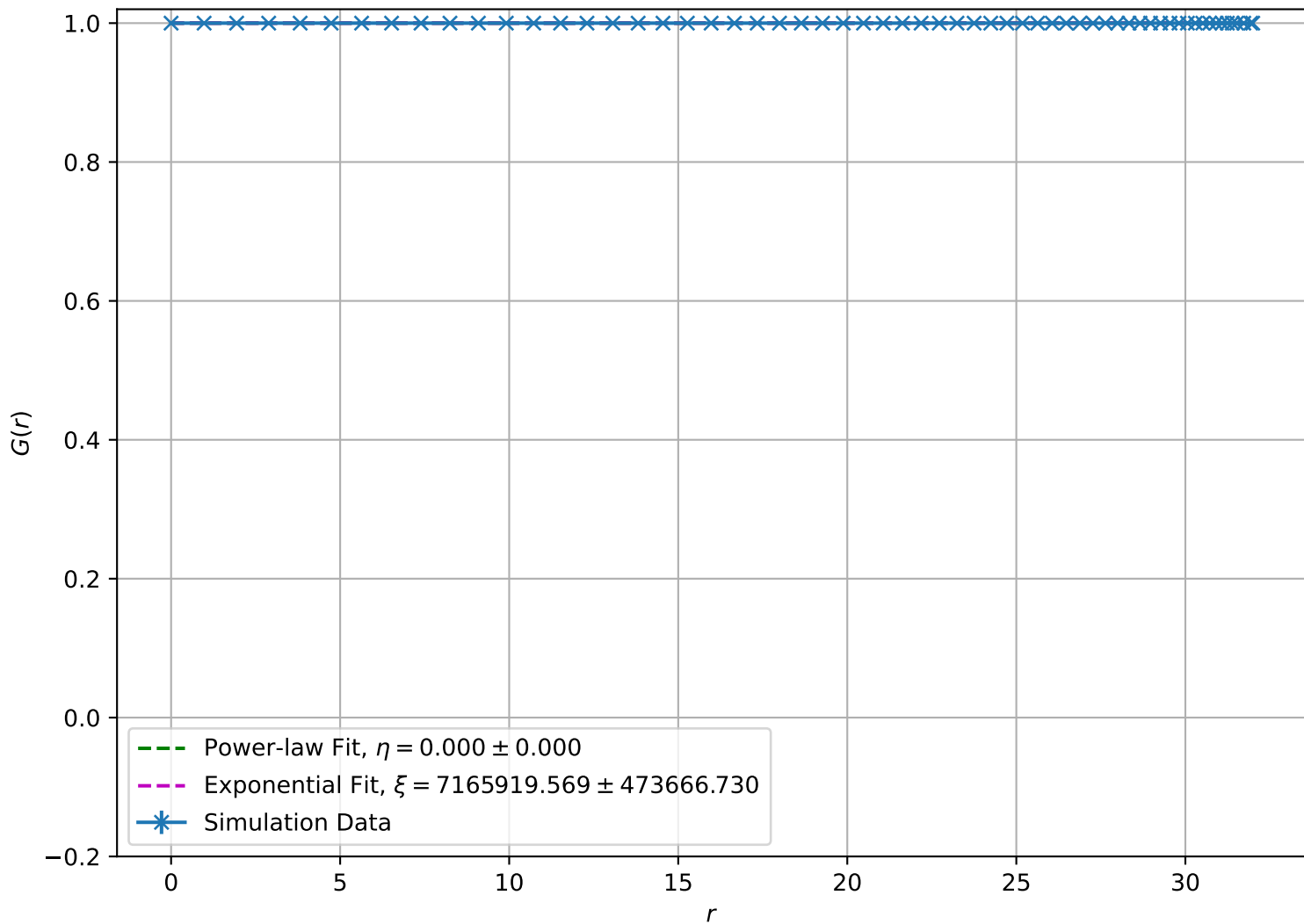
Correlation Function at T = 1.00\text{e} - 05 , L = 32
