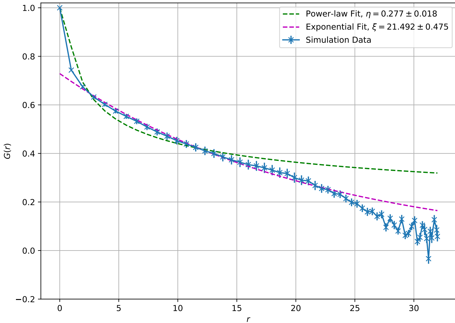
Correlation Function at T = 1.10e + 00 , L = 32
