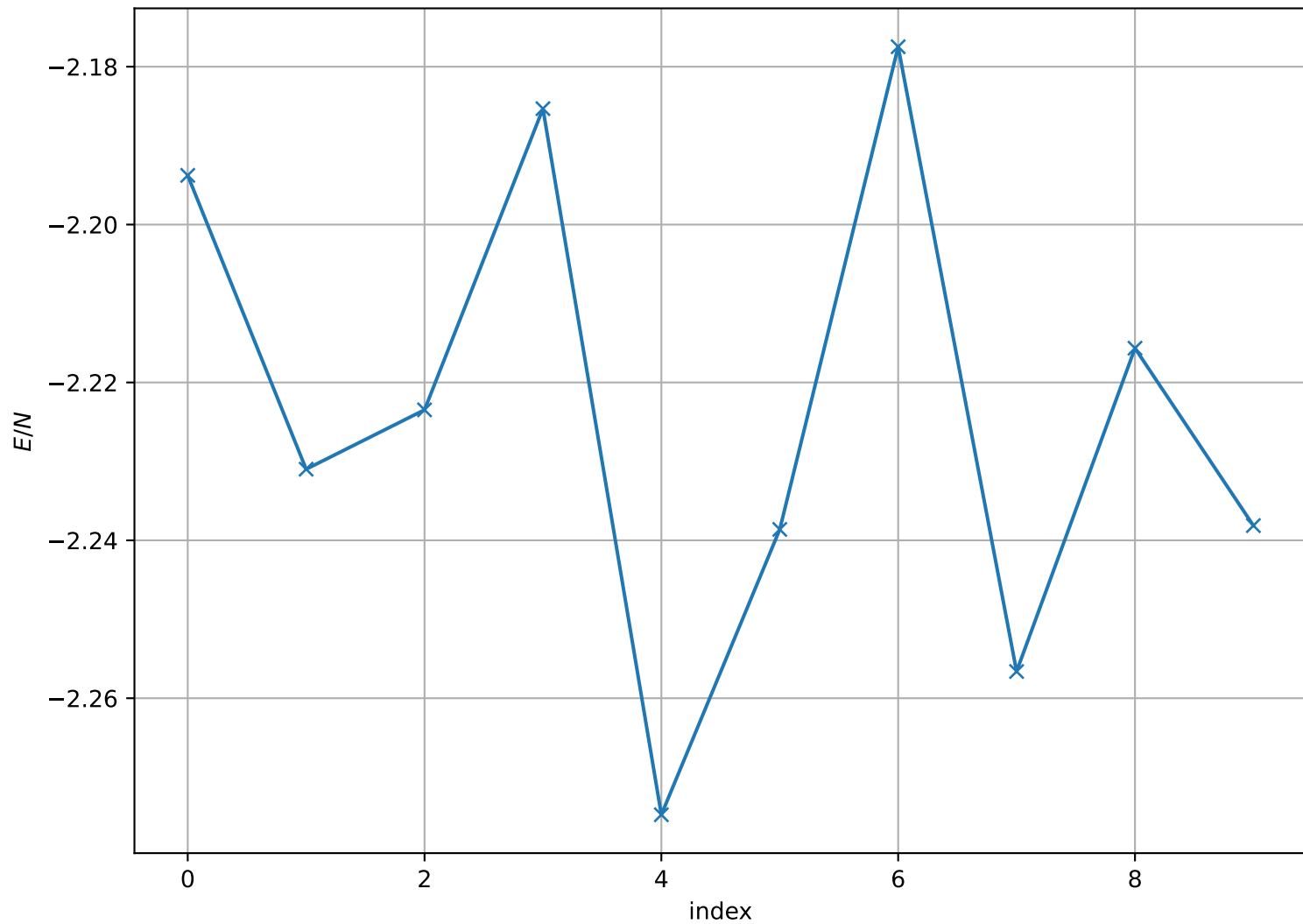
Energy per Site at T = 1.100e + 00 , L = 32
