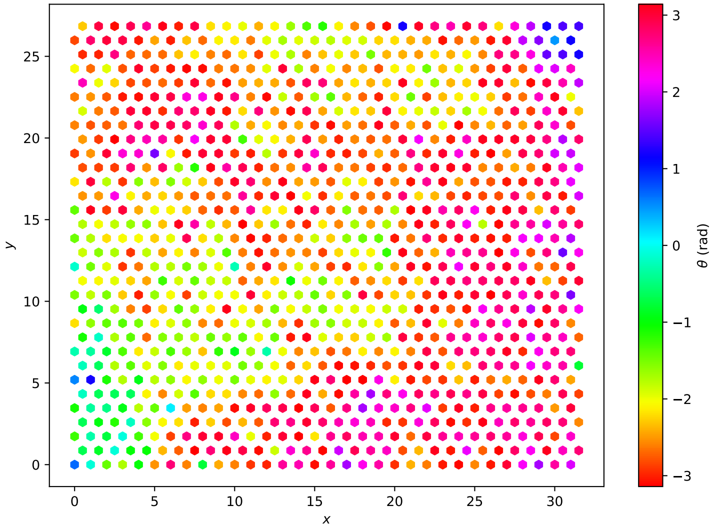
Hexagonal Lattice L=32 , T = 1.10e + 00
