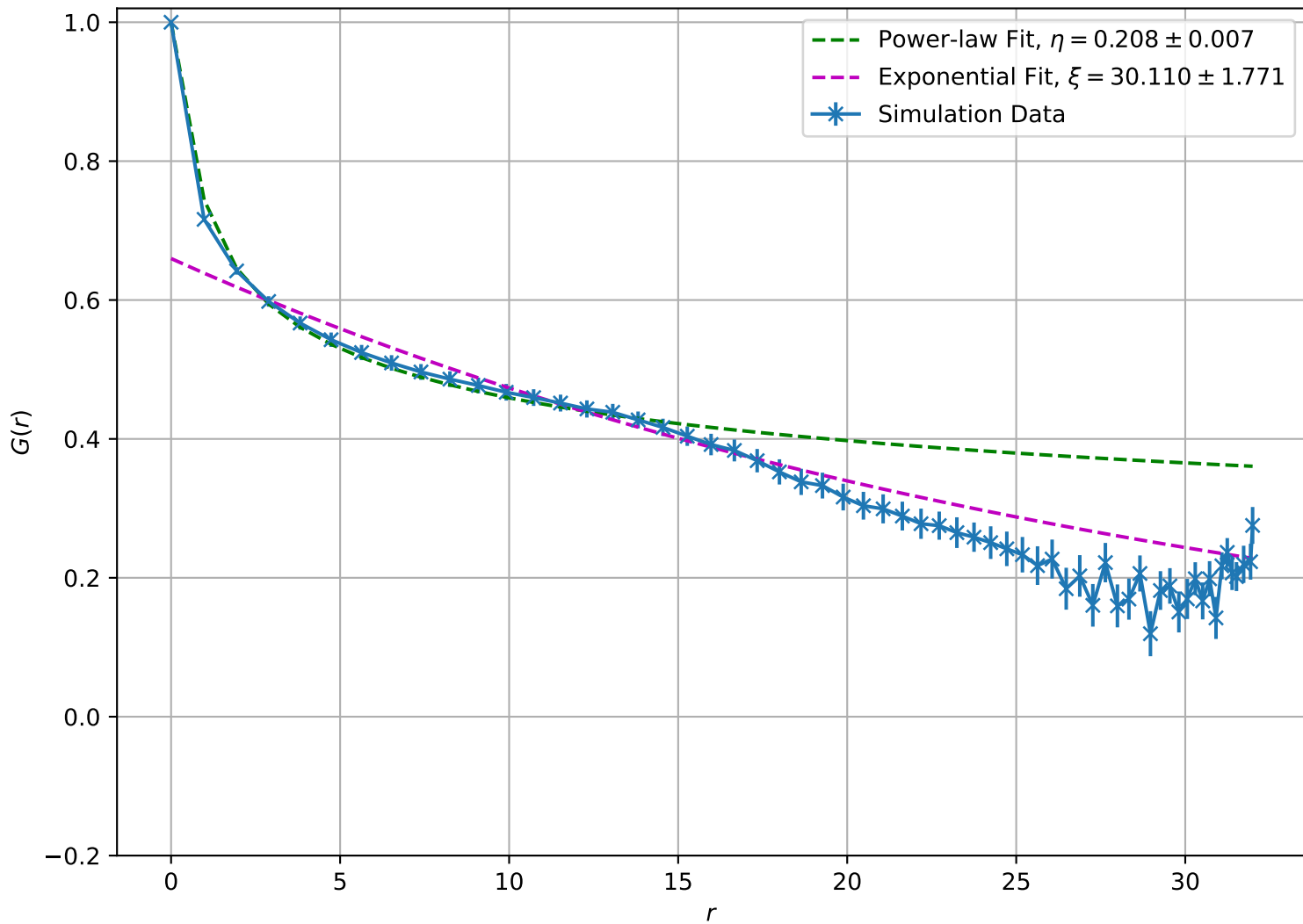
Correlation Function at T = 1.20\text{e} + 00 , L = 32
