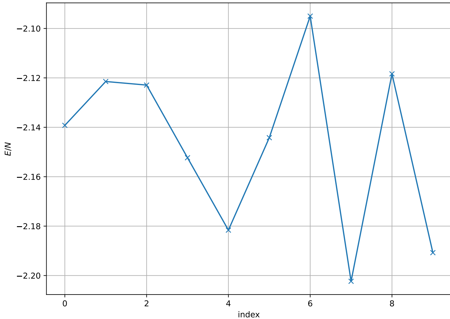
Energy per Site at T = 1.200e + 00 , L = 32
