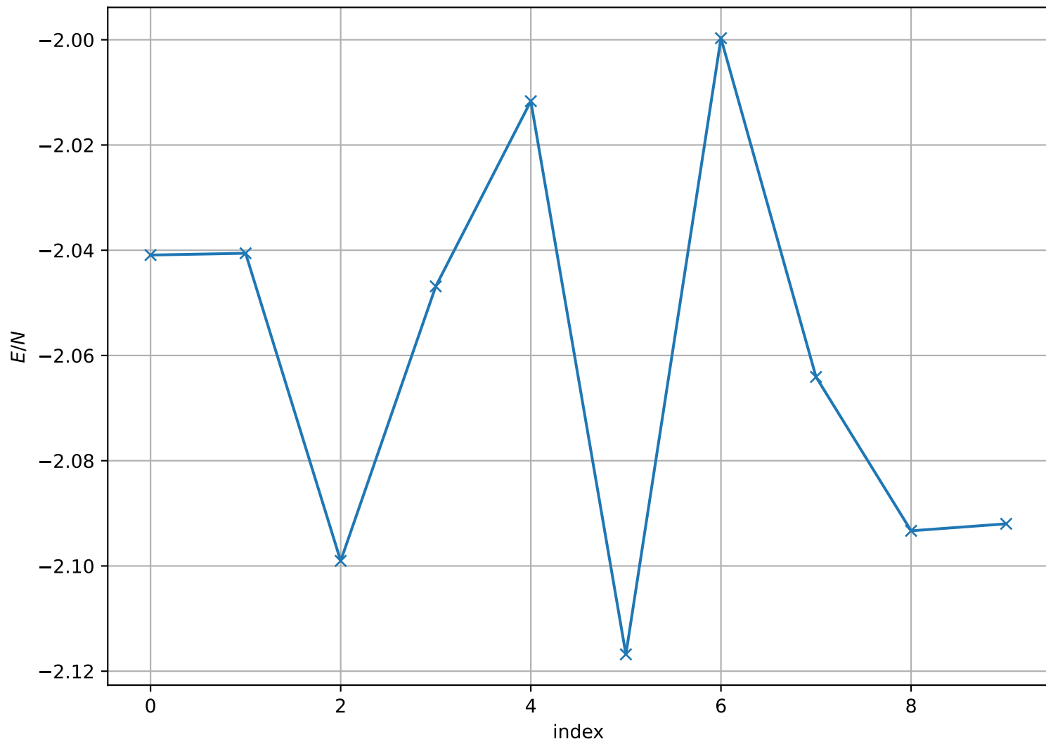
Energy per Site at T = 1.300e + 00 , L = 32
