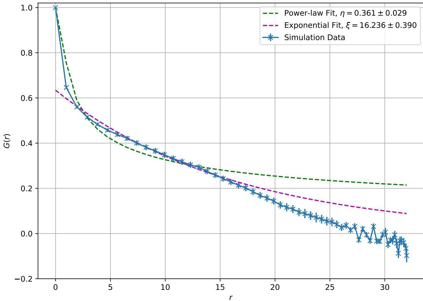
Correlation Function at T = 1.40e + 00 , L = 32
