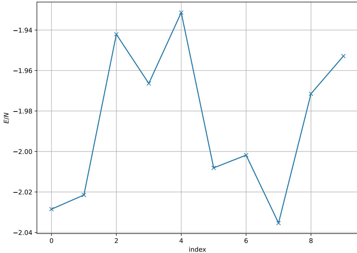
Energy per Site at T = 1.400e + 00 , L = 32
