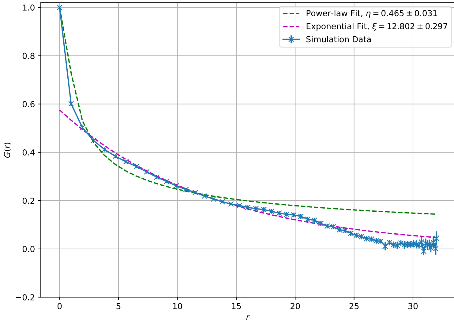
Correlation Function at T = 1.50e + 00 , L = 32
