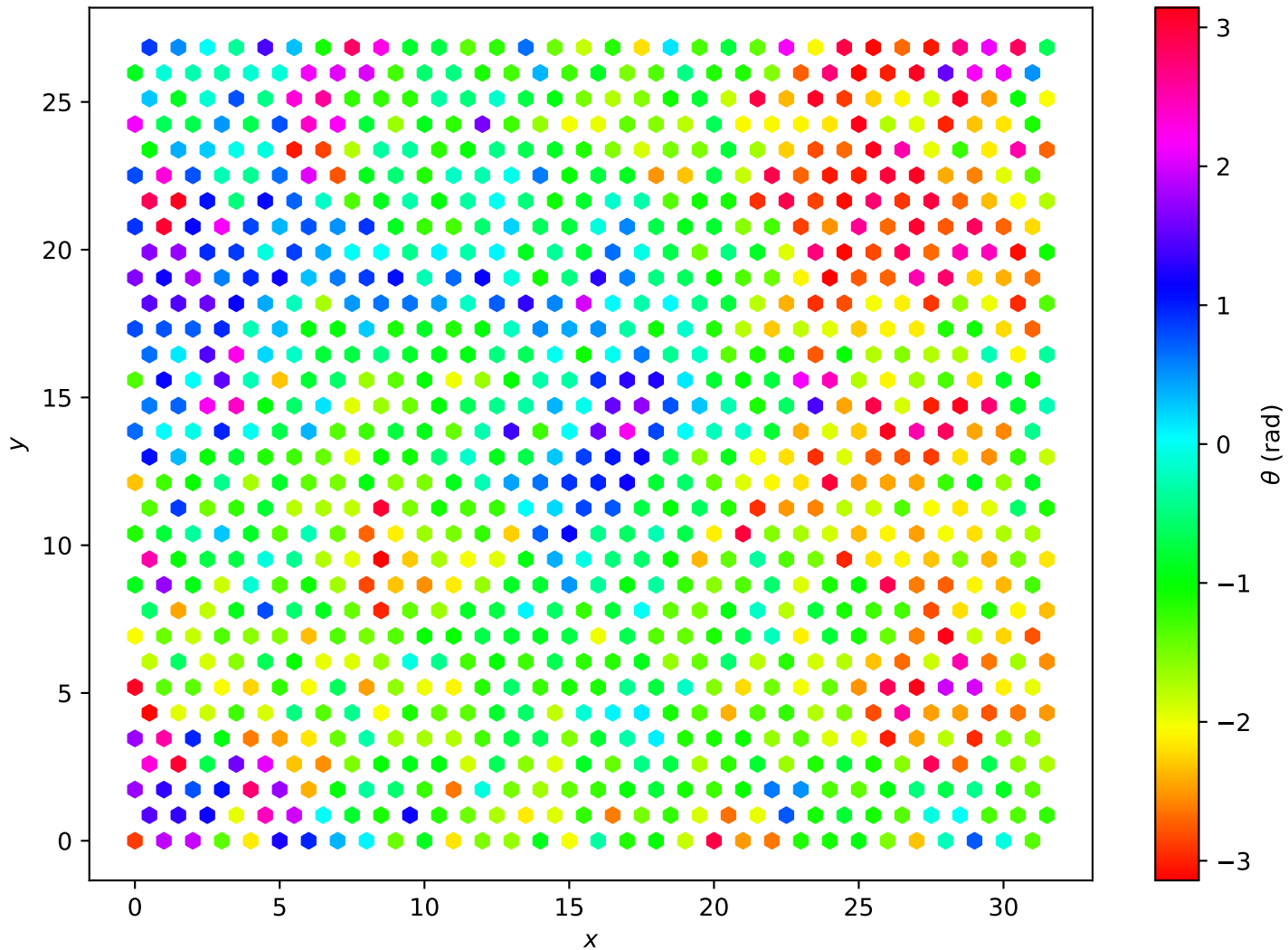
Hexagonal Lattice L=32 , T = 1.50e + 00
