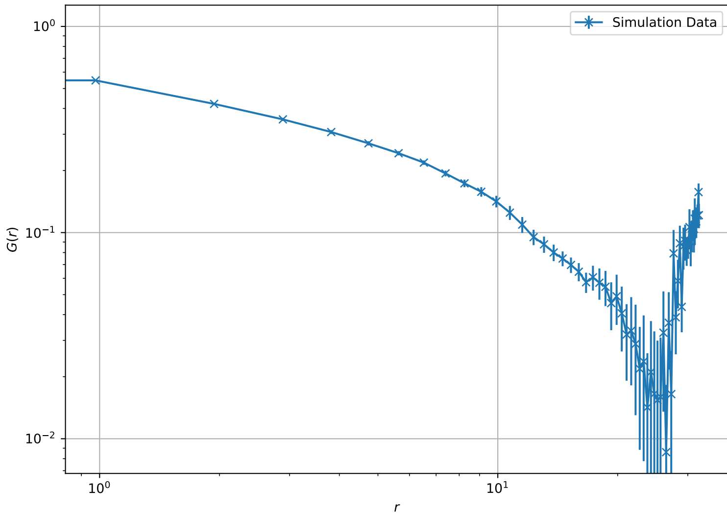
Correlation Function at T = 1.60e + 00 , L = 32 (Log-Log Scale)
