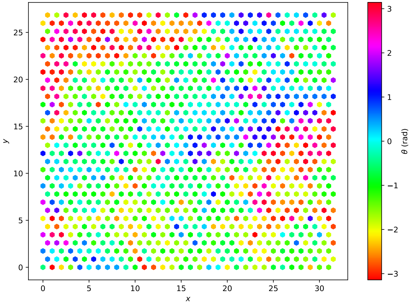
Hexagonal Lattice L=32 , T = 1.60e + 00
