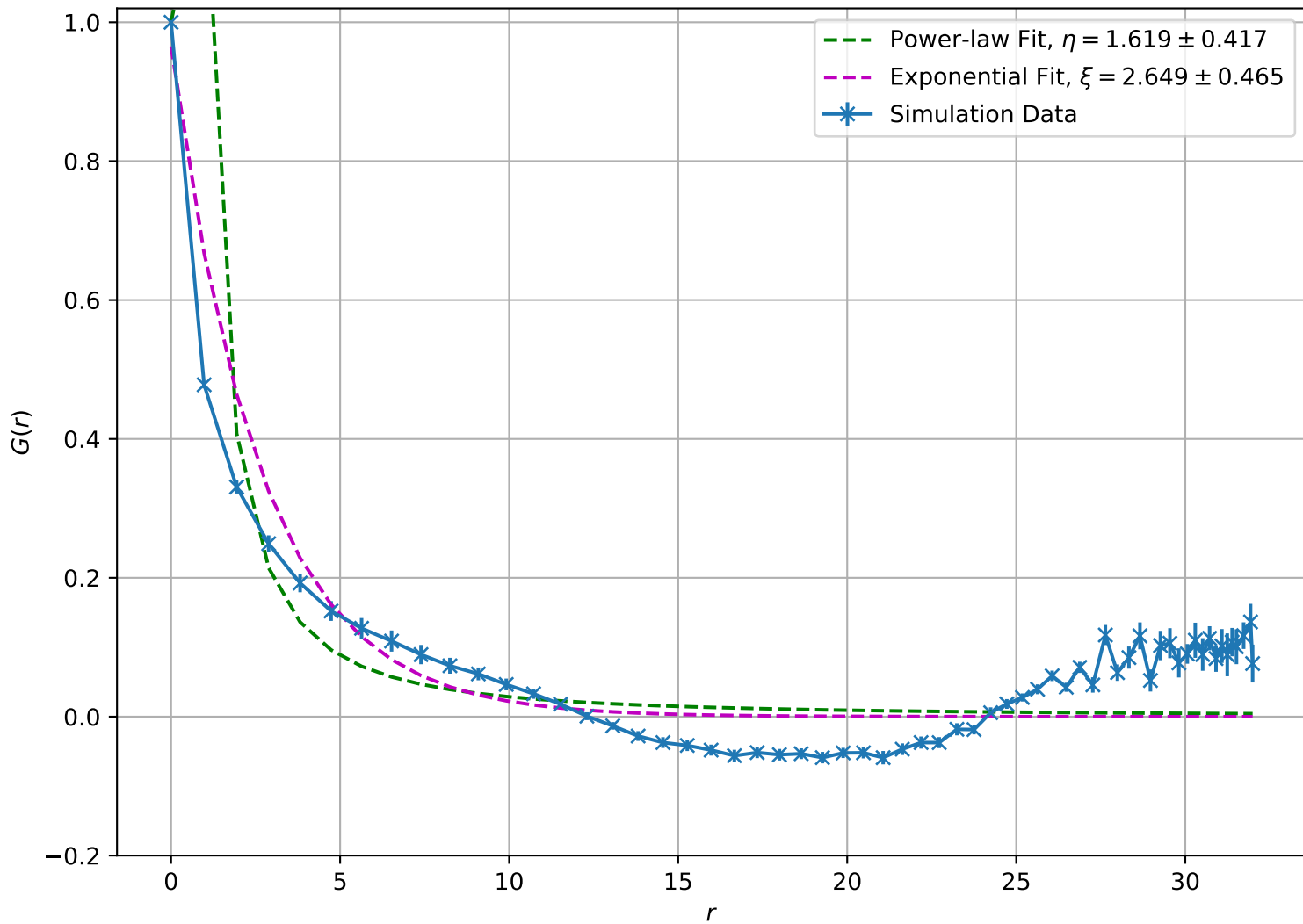
Correlation Function at T = 1.70e + 00 , L = 32
