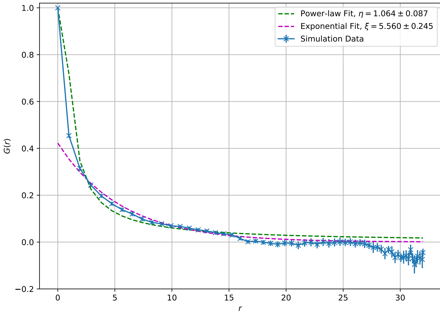
Correlation Function at T = 1.80\text{e} + 00 , L = 32
