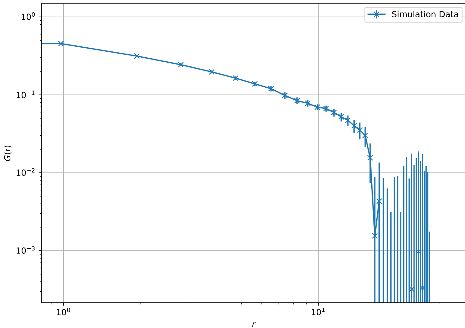
Correlation Function at T = 1.80e + 00 , L = 32 (Log-Log Scale)
