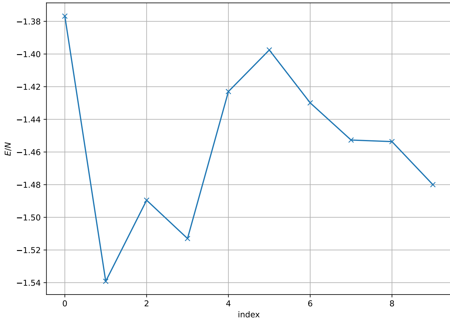
Energy per Site at T = 1.800e + 00 , L = 32
