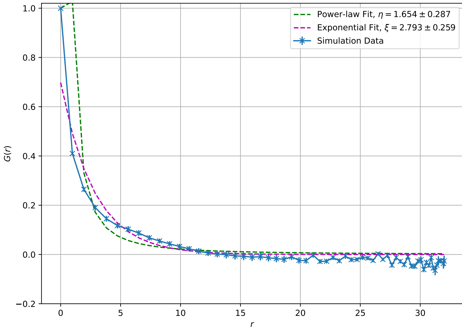
Correlation Function at T = 1.90e + 00 , L = 32
