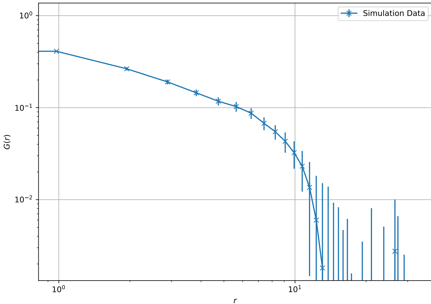
Correlation Function at T = 1.90e + 00 , L = 32 (Log-Log Scale)
