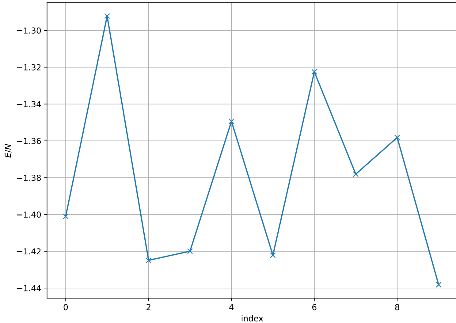
Energy per Site at T = 1.900e + 00 , L = 32
