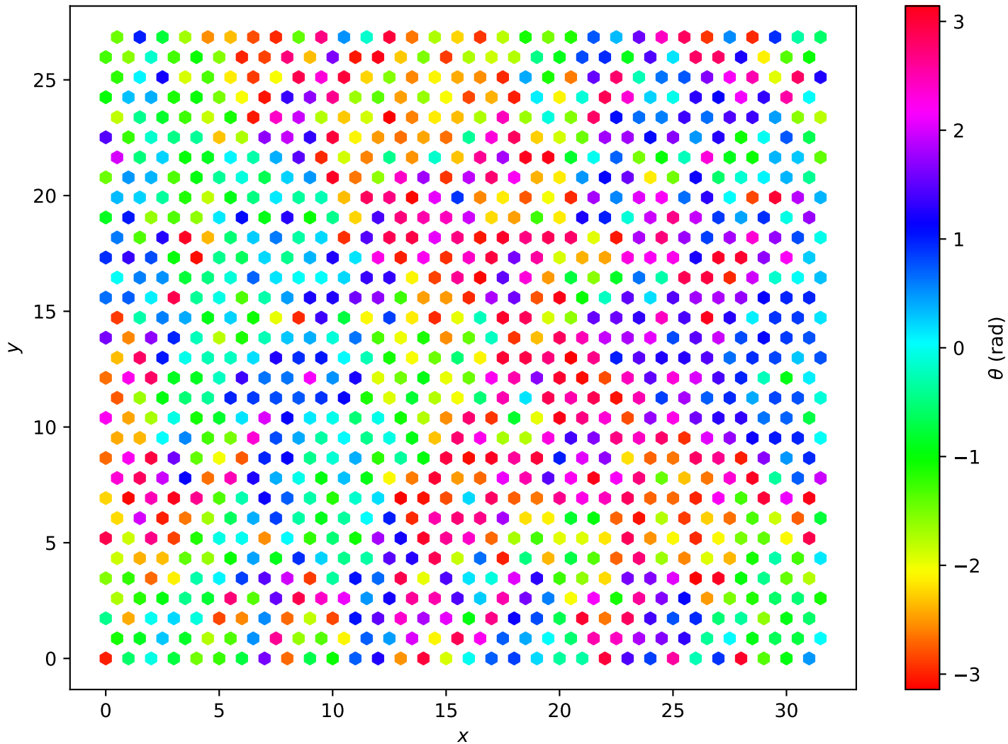
Hexagonal Lattice L=32 , T = 1.90e + 00
