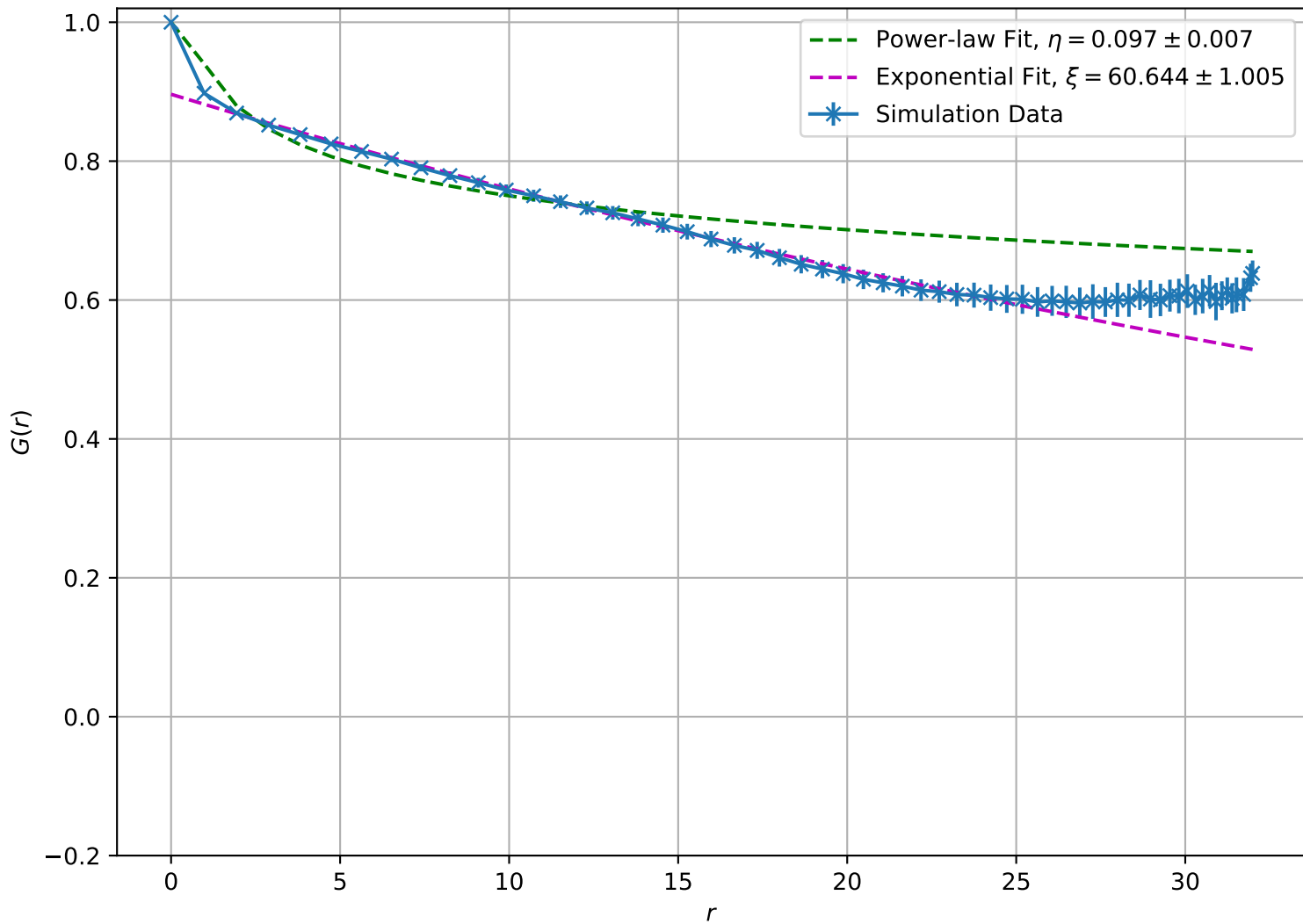
Correlation Function at T = 5.00e - 01 , L = 32
