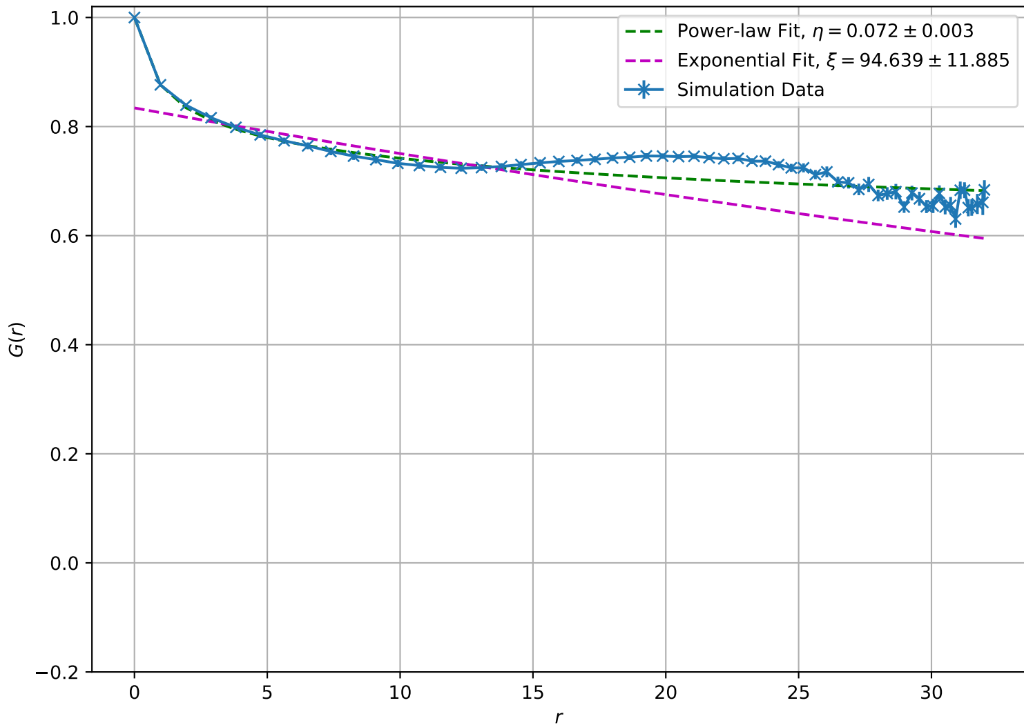
Correlation Function at T = 6.00e - 01 , L = 32
