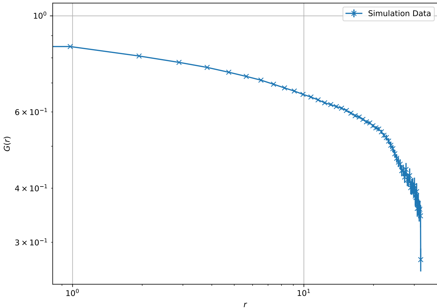
Correlation Function at T = 7.00e - 01 , L = 32 (Log-Log Scale)
