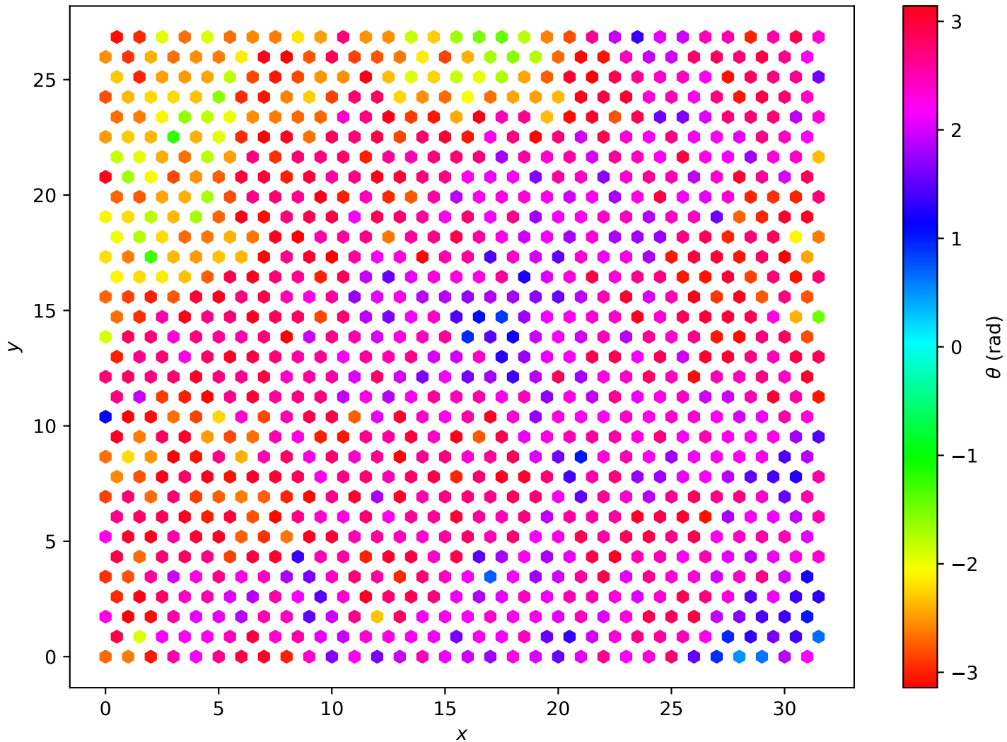
Hexagonal Lattice L=32 , T = 7.00e - 01
