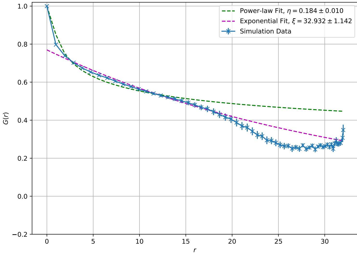
Correlation Function at T = 9.00\text{e} - 01 , L = 32
