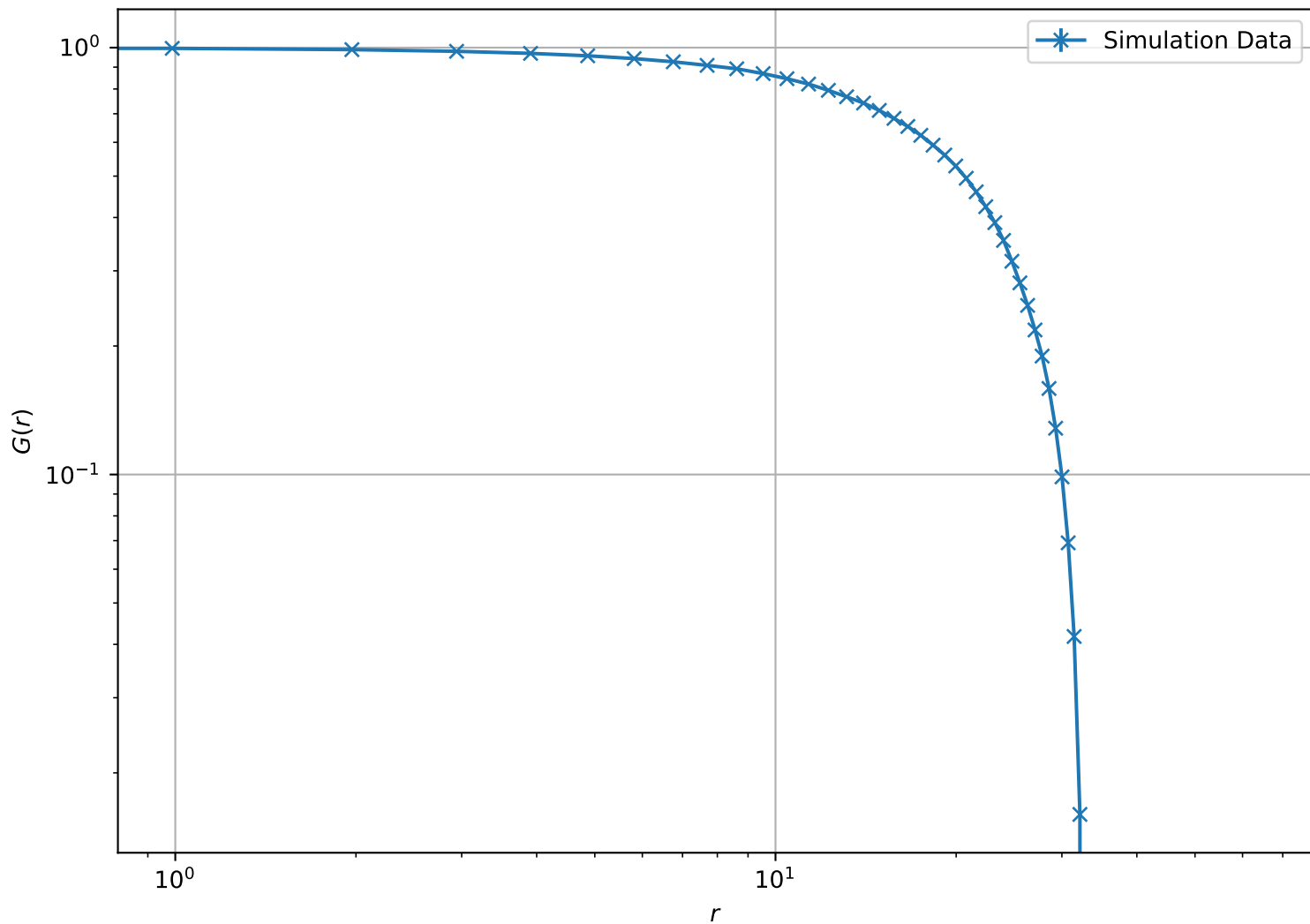
Correlation Function at T = 1.00\text{e} - 05 , L = 64 (Log-Log Scale)
