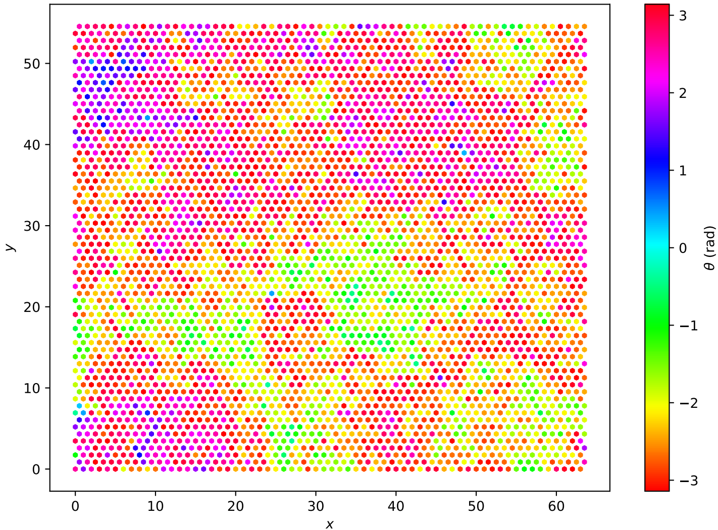
Hexagonal Lattice L=64 , T = 1.10e + 00
