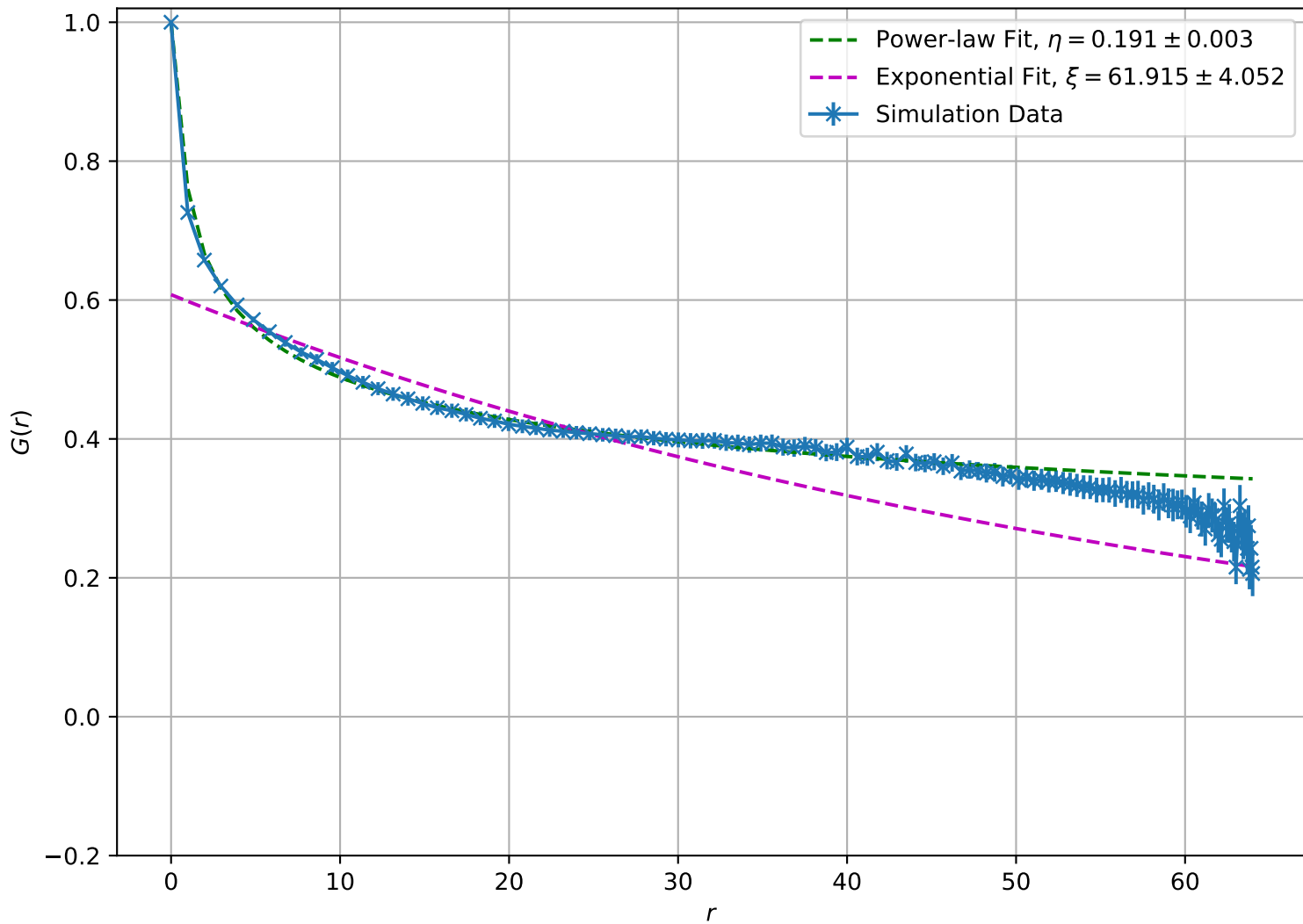
Correlation Function at T = 1.20\text{e} + 00 , L = 64
