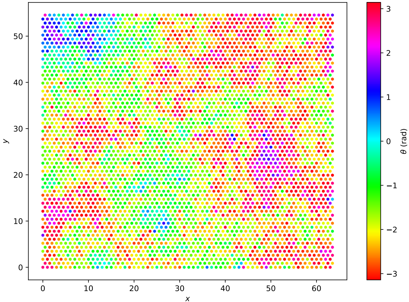
Hexagonal Lattice L=64 , T = 1.20e + 00
