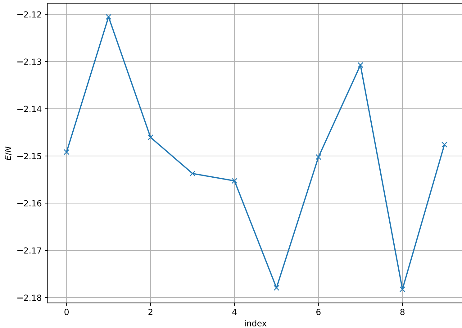
Energy per Site at T = 1.300e + 00 , L = 64
