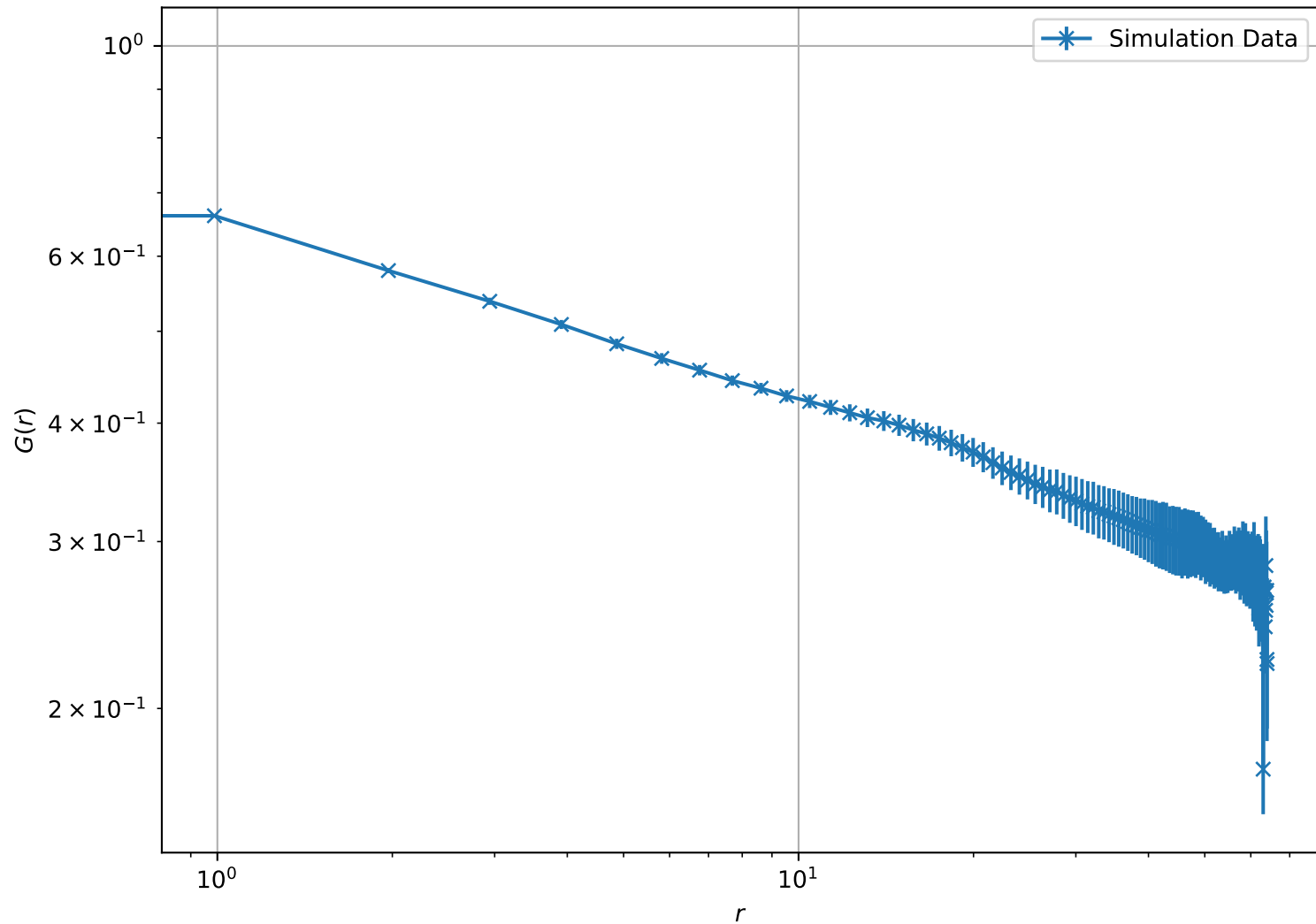
Correlation Function at T = 1.40e + 00 , L = 64 (Log-Log Scale)
