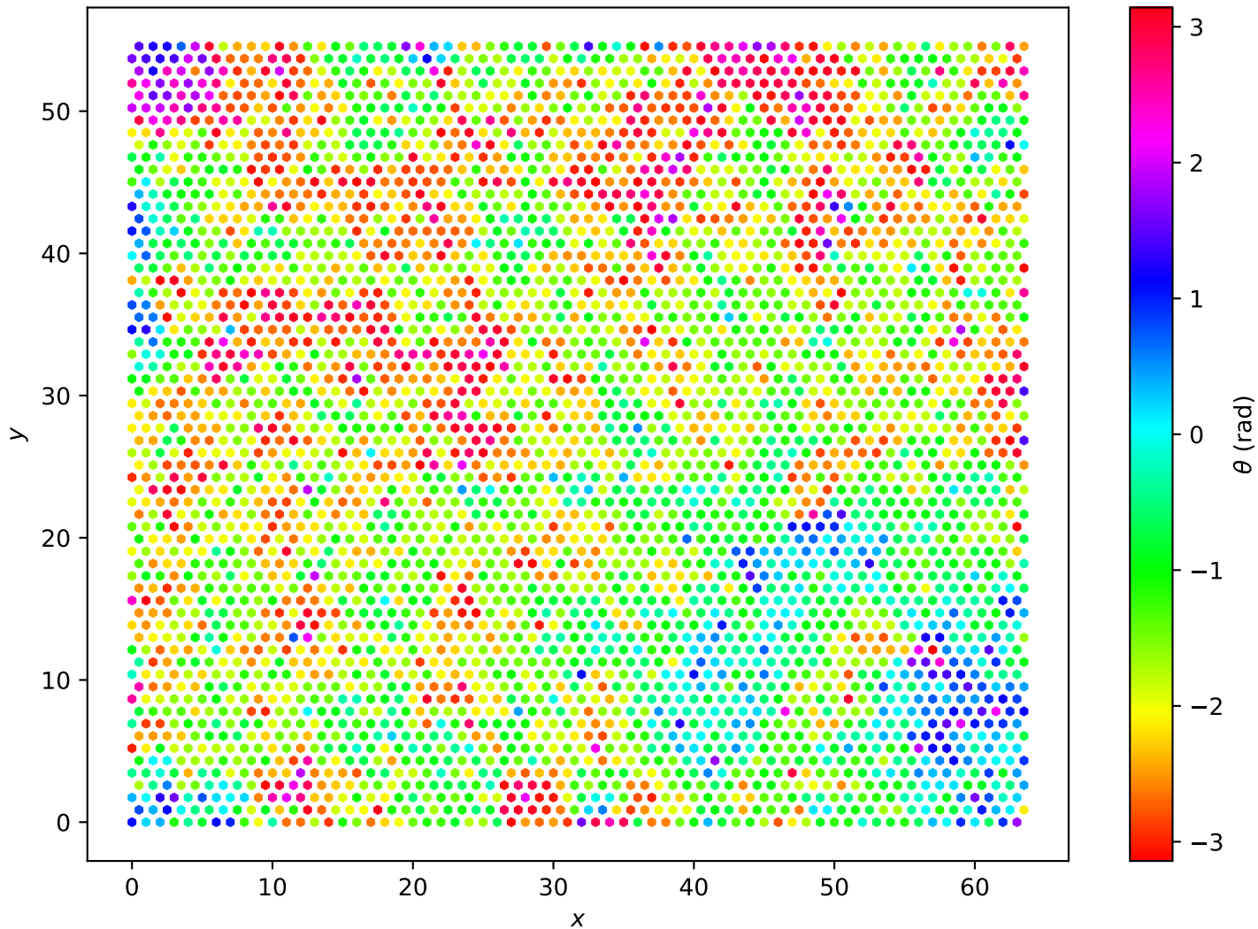
Hexagonal Lattice L=64 , T = 1.40e + 00
